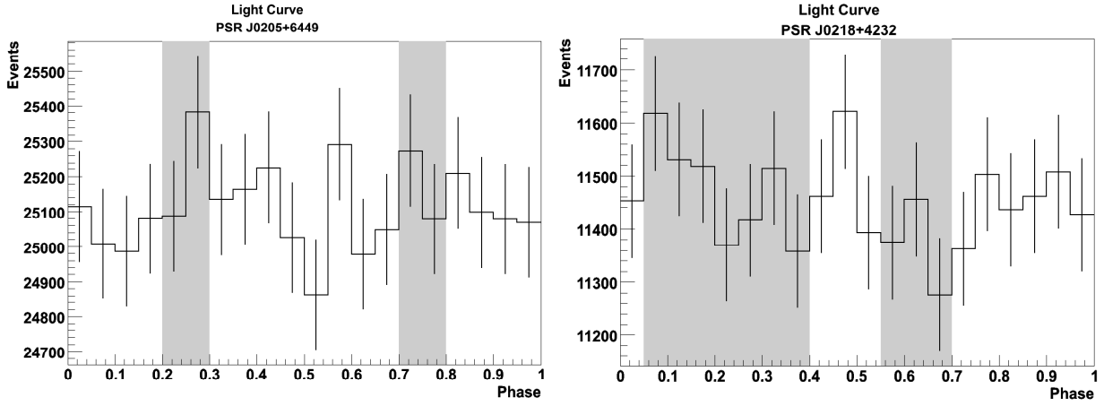
FIG. 3.— Left: Light curve at PSR J0205+6449 for 80 \text{ GeV} < E < 300 \text{ GeV} ( E_{th} \sim 180 \text{ GeV} ). The shadowed area corresponds to the RXTE pulse peaks (Ransom et al. 2004). 0.1\sigma signal significance for the H-test. Right: Light curve for PSR J0218+4232 for low energies ( 50 < E < 300 \text{ GeV} ; E_{th} \sim 120 \text{ GeV} ). The shadowed area corresponds to the EGRET pulse peaks (Kuiper et al. 2002). Signal significance (H-test) \sim 0.6\sigma .
