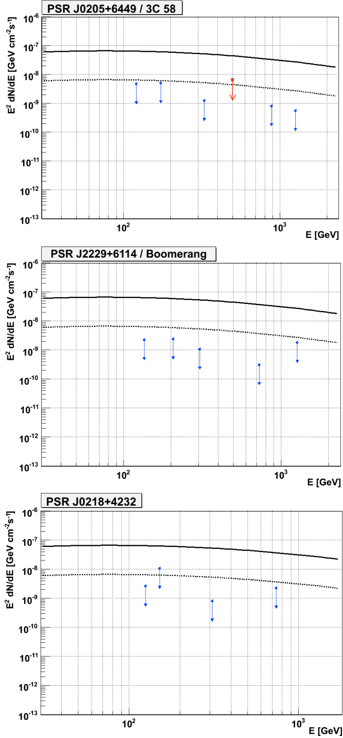
FIG. 2.— DC Flux upper limits (99% c.l.) for the three pulsars and their corresponding nebulae from MAGIC observations (blue arrows): On top, 3C58 and PSR J0205+6449; in the middle, Boomerang and PSR J2229+6114; and at the bottom, PSR J0218+4232. The black lines denote different fractions of the Crab flux: dashed line shows 10% and solid line 100% of the Crab flux. The red filled square is the upper limit obtained from Whipple observations of 3C 58 (Hall et al. 2001).
