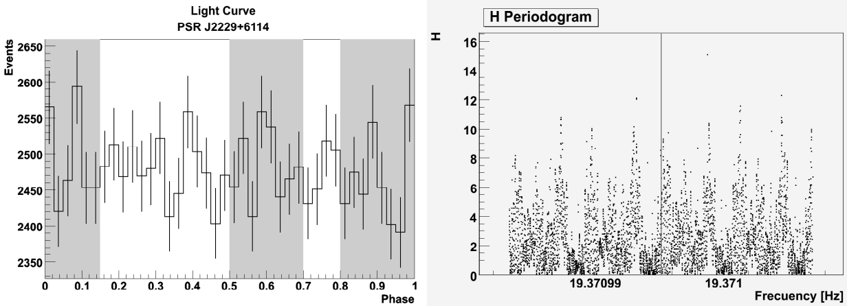
FIG. 4.— Left: Light curve for PSR J2229+6114 at energies: 70 < E < 300 \text{ GeV} , E_{th} \sim 135 \text{ GeV} for the ephemeris frequency. The shadowed area corresponds to the ASCA GIS pulse peaks (0.8-10 keV) (Halpern et al. 2001). Signal significance \sim 0.2 \sigma for H-test. Right: Periodogram for the H-test for the frequencies scan. The central frequency is the corresponding one in radio wavelength.
