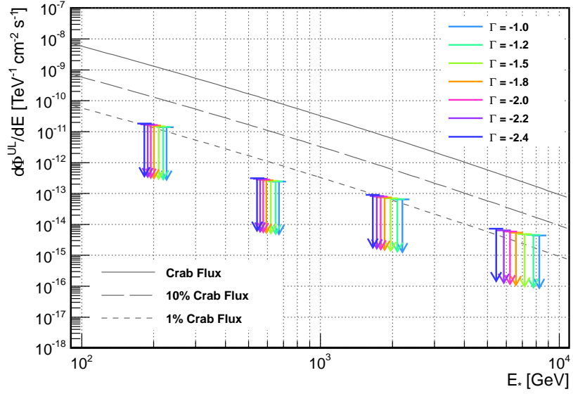
Figure 18: Differential flux upper limits from 157.9 hours of the Segue 1 observations with MAGIC, assuming a point-like source and a power law-shaped signal emission and different spectral slopes \Gamma . As a reference, the Crab Nebula differential flux (solid line, [46]) and its 10% and 1% fractions (long-dashed and dashed lines, respectively), are also drawn.
