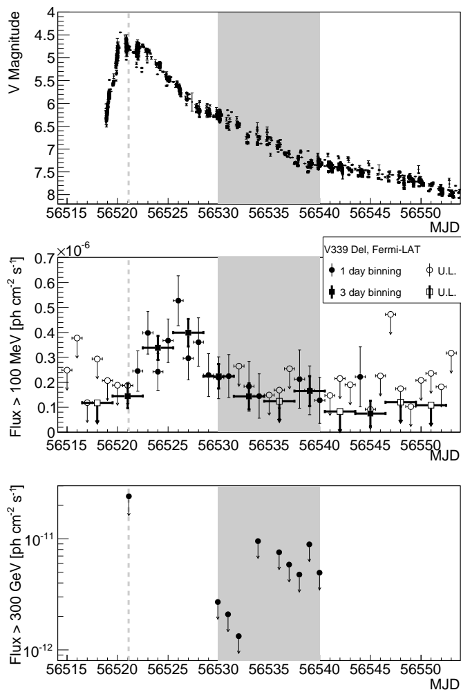
Fig. 1. Multi-wavelength light curve of V339 Del during the outburst in August 2013. Top panel: Optical observations in the V band obtained from the AAVSO-LCG a service. Middle panel: The Fermi -LAT flux (filled symbols) and upper limits (empty symbols) above 100 MeV in 1-day (circles, thin lines) or 3-day (squares, thick lines) bins. A 95% C.L. flux upper limit is shown for time bins with TS < 4 . Bottom panel: Upper limit on the flux above 300 GeV observed with MAGIC telescopes. The gray band shows the observation nights with MAGIC. The dashed gray line shows a MAGIC observation night affected by bad weather.
